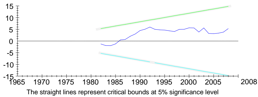
Plot of Cumulative Sum of Recursive Residuals
